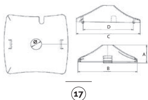
CPG plastic cover for swivel frame
